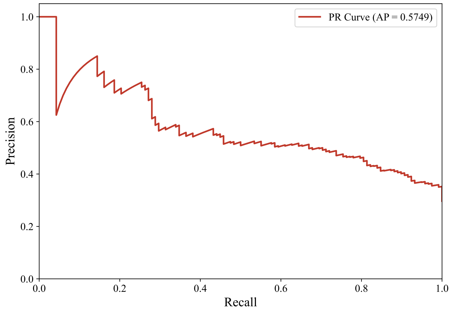
Precision-Recall Curve — DUTCH_MANUAL (bert-base-multilingual-uncased, Voting_Ensemble)
