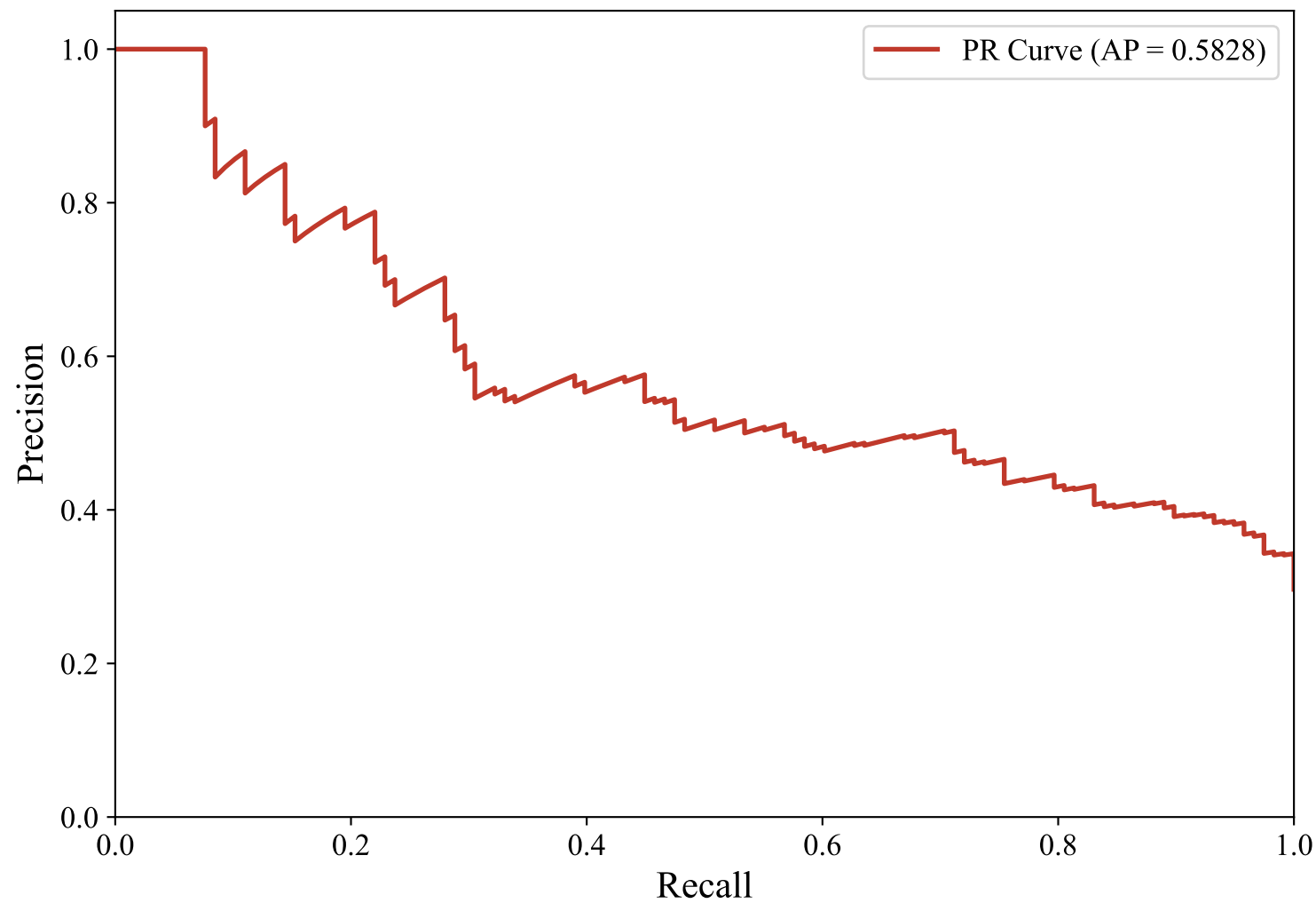
Precision-Recall Curve — DUTCH_MANUAL (bert-base-multilingual-uncased, XGBoost)
