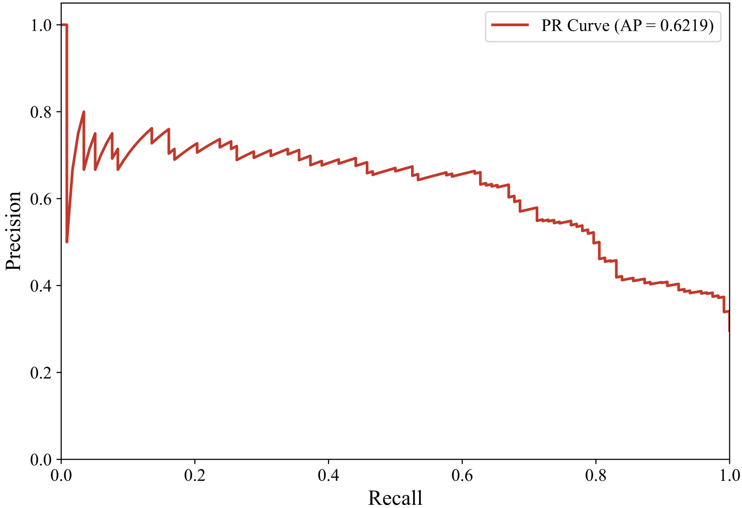
Precision-Recall Curve — DUTCH_MANUAL (xlm-roberta-base, XGBoost)
