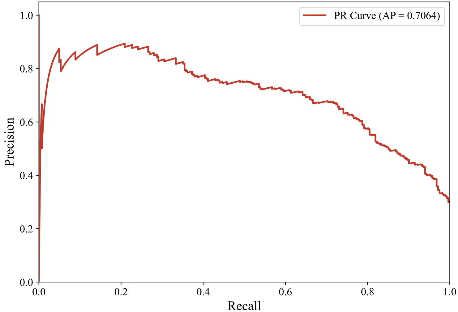
Precision-Recall Curve — ENGLISH_MANUAL (bert-base-multilingual-uncased, LightGBM)
