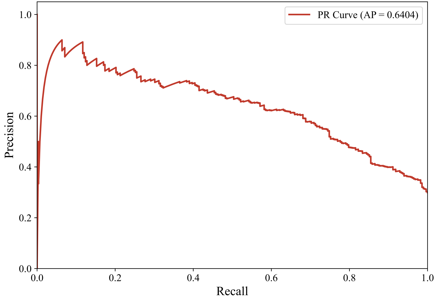
Precision-Recall Curve — ENGLISH_MANUAL (bert-base-multilingual-uncased, Random_Forest)
