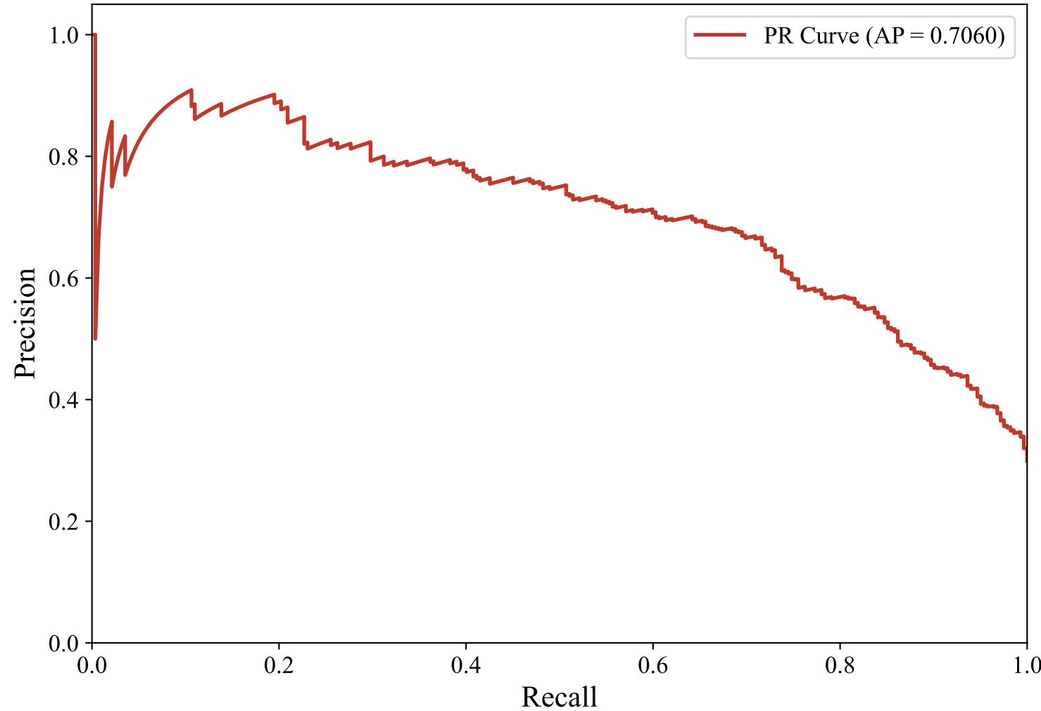
Precision-Recall Curve — ENGLISH_MANUAL (bert-base-multilingual-uncased, XGBoost_Optimized)
