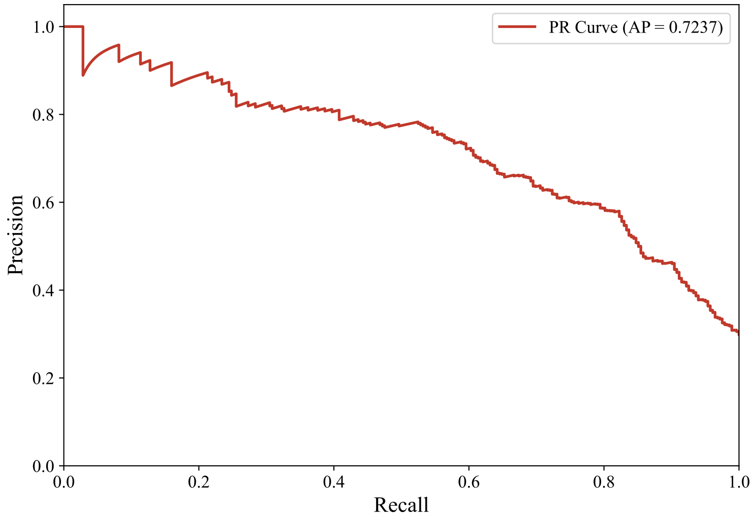
Precision-Recall Curve — ENGLISH_MANUAL (paraphrase-multilingual-mpnet-base-v2, Random_Forest)
