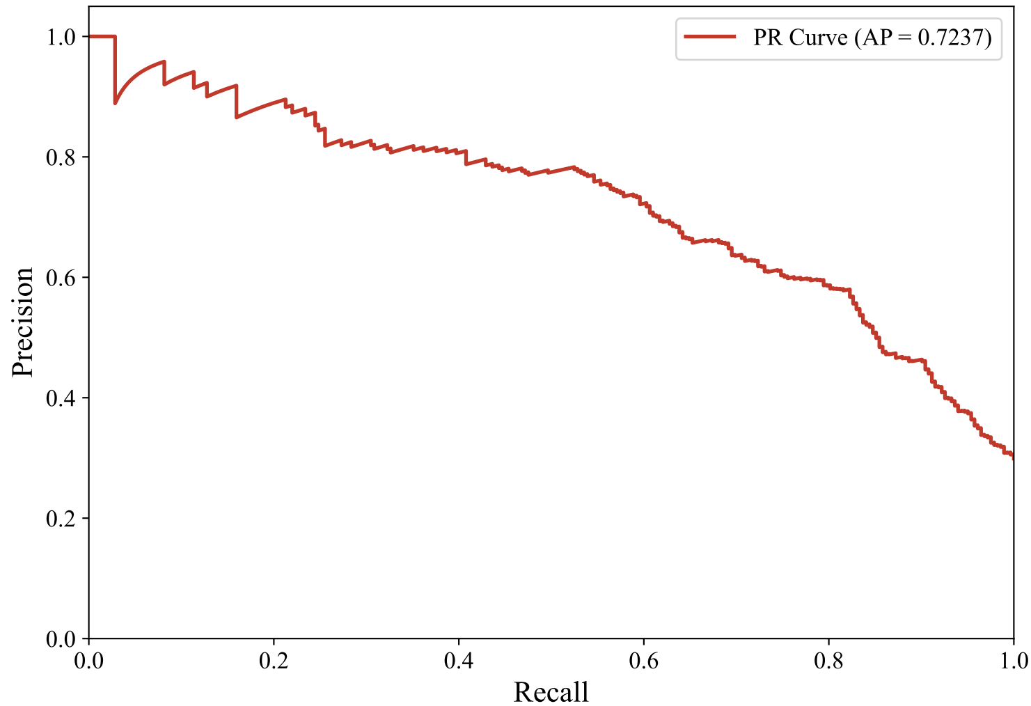
Precision-Recall Curve — ENGLISH_MANUAL (paraphrase-multilingual-mpnet-base-v2, Random_Forest_Optimized)
