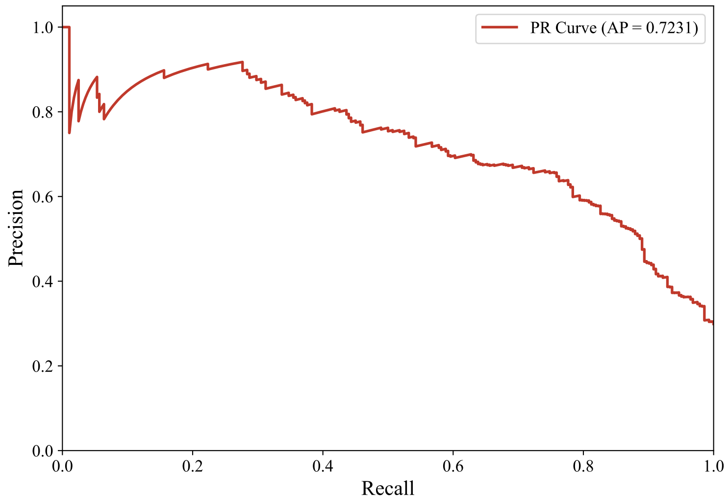
Precision-Recall Curve — ENGLISH_MANUAL (xlm-roberta-base, LightGBM_Optimized)
