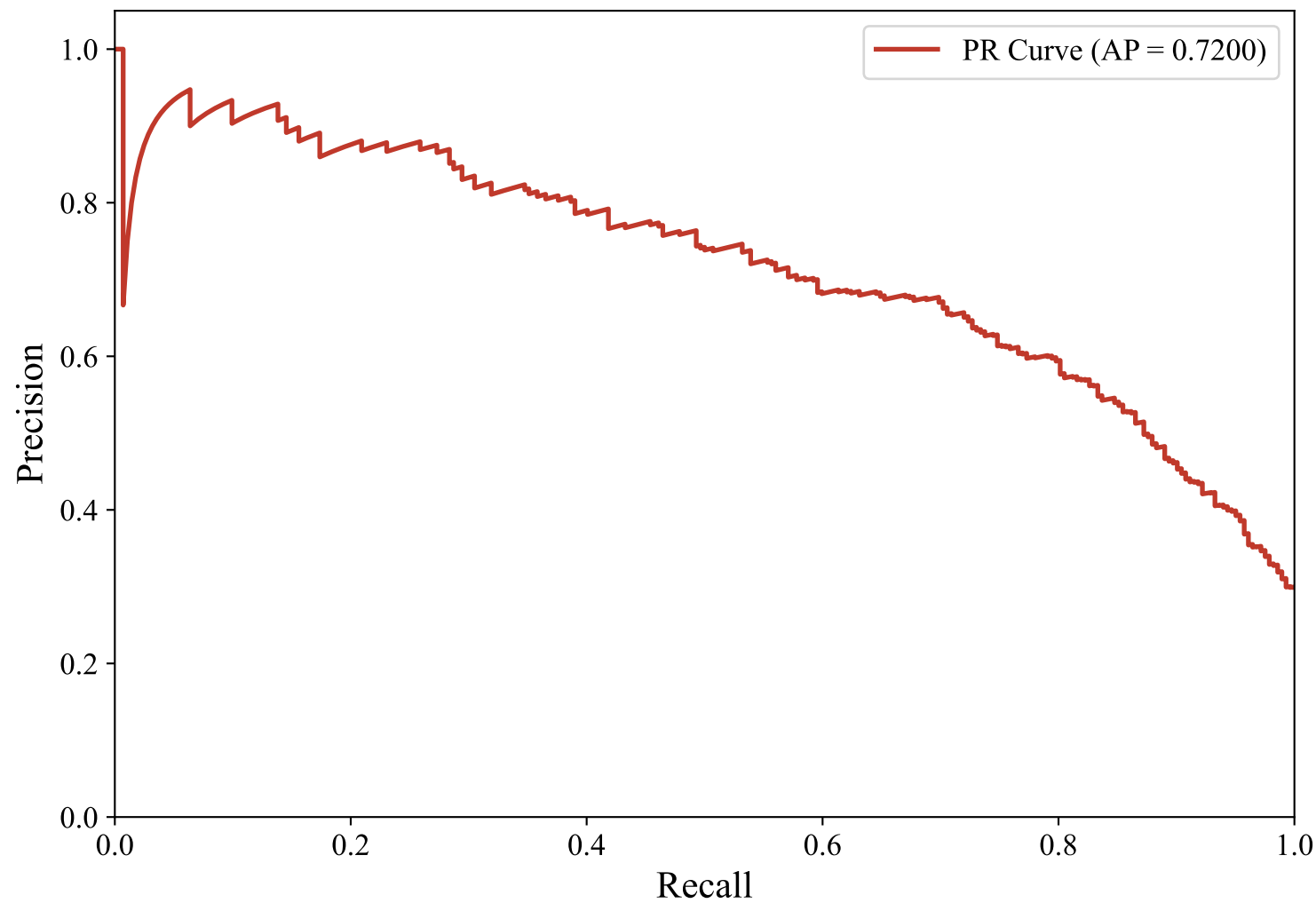
Precision-Recall Curve — ENGLISH_MANUAL (xlm-roberta-base, XGBoost_Optimized)
