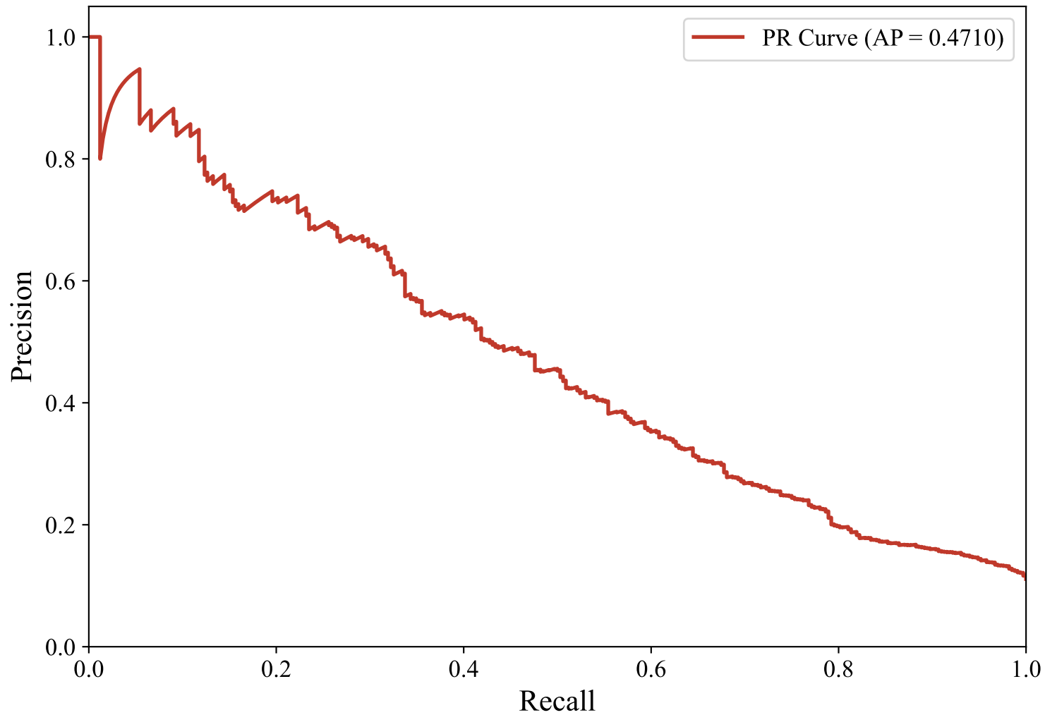
Precision-Recall Curve — GERMAN_MANUAL (paraphrase-multilingual-mpnet-base-v2, LightGBM_Optimized)
