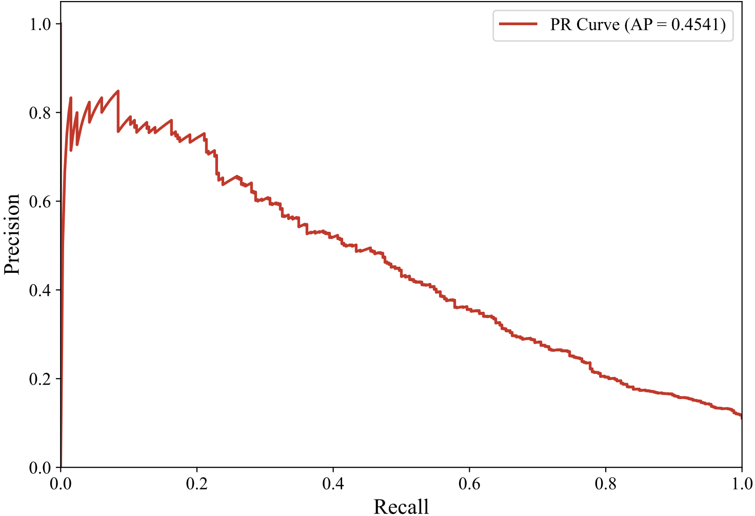
Precision-Recall Curve — GERMAN_MANUAL (paraphrase-multilingual-mpnet-base-v2, Voting_Ensemble)
