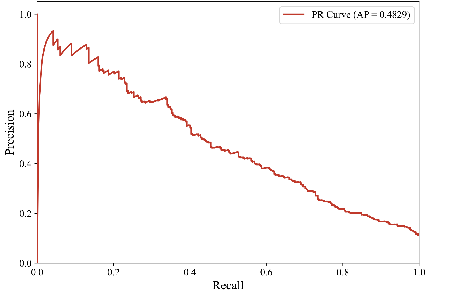
Precision-Recall Curve — GERMAN_MANUAL (paraphrase-multilingual-mpnet-base-v2, XGBoost)
