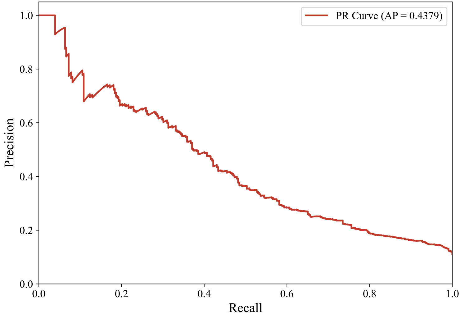
Precision-Recall Curve — GERMAN_MANUAL (xlm-roberta-base, Random_Forest)
