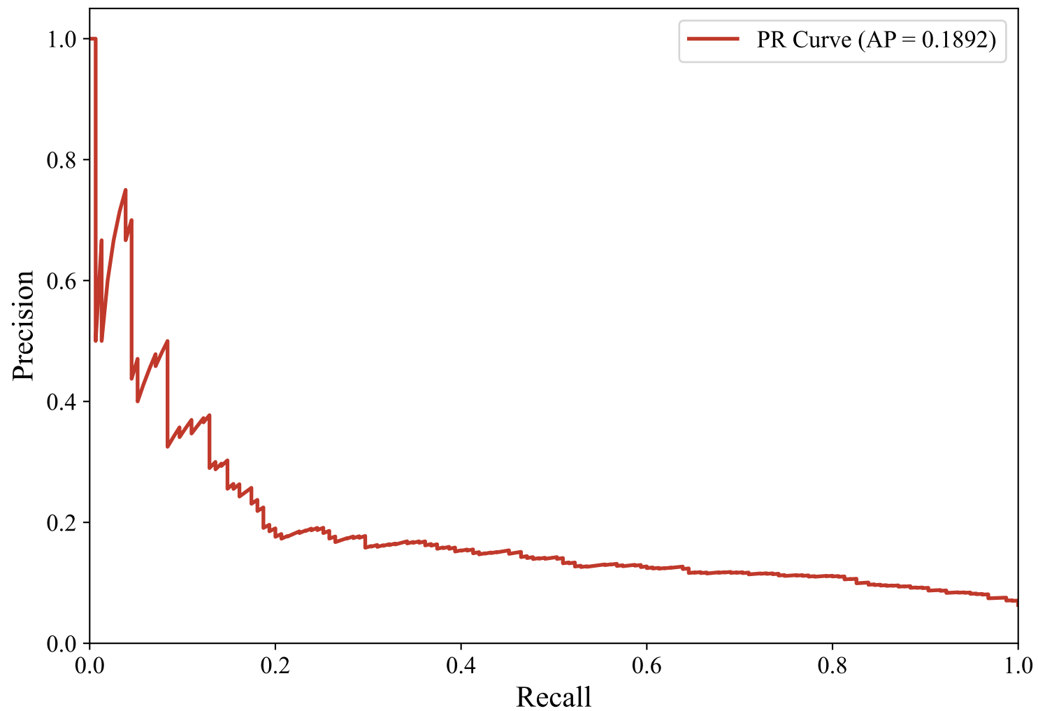
Precision-Recall Curve — SWEDISH_MANUAL (bert-base-multilingual-uncased, LightGBM)
