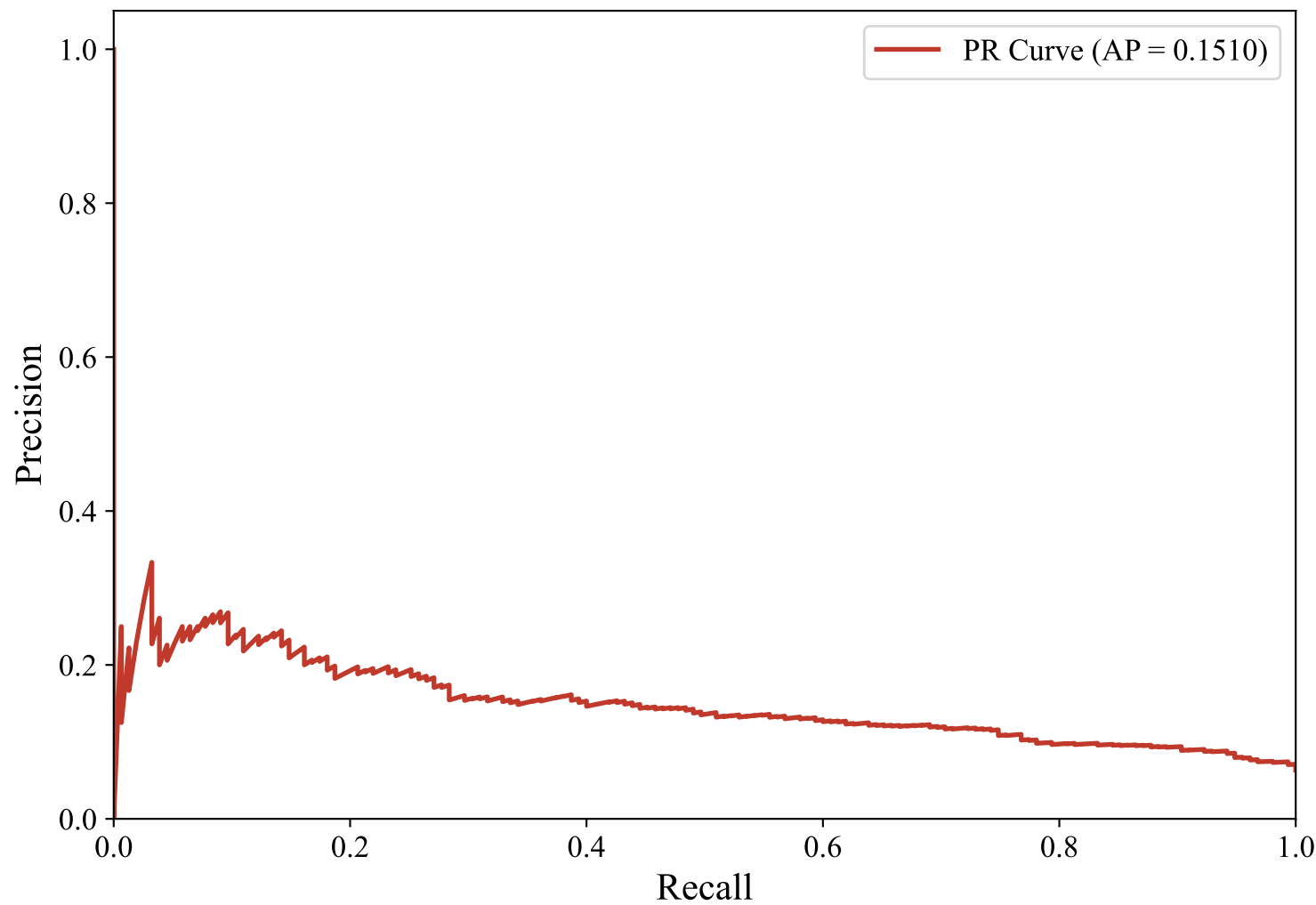
Precision-Recall Curve — SWEDISH_MANUAL (bert-base-multilingual-uncased, Random_Forest)
