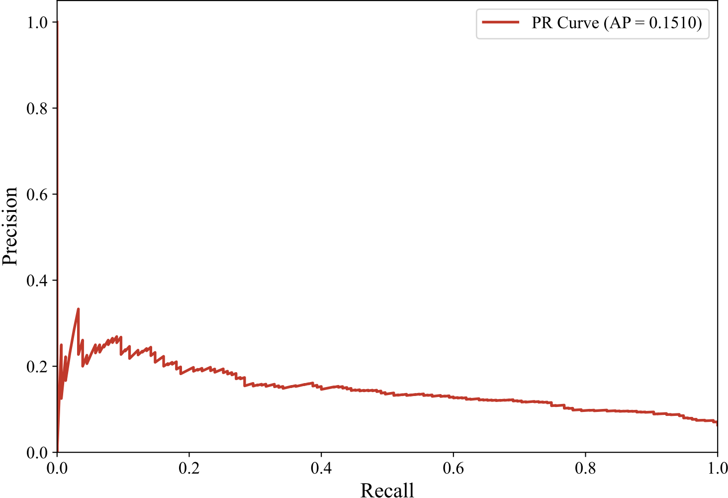
Precision-Recall Curve — SWEDISH_MANUAL (bert-base-multilingual-uncased, Random_Forest_Optimized)
