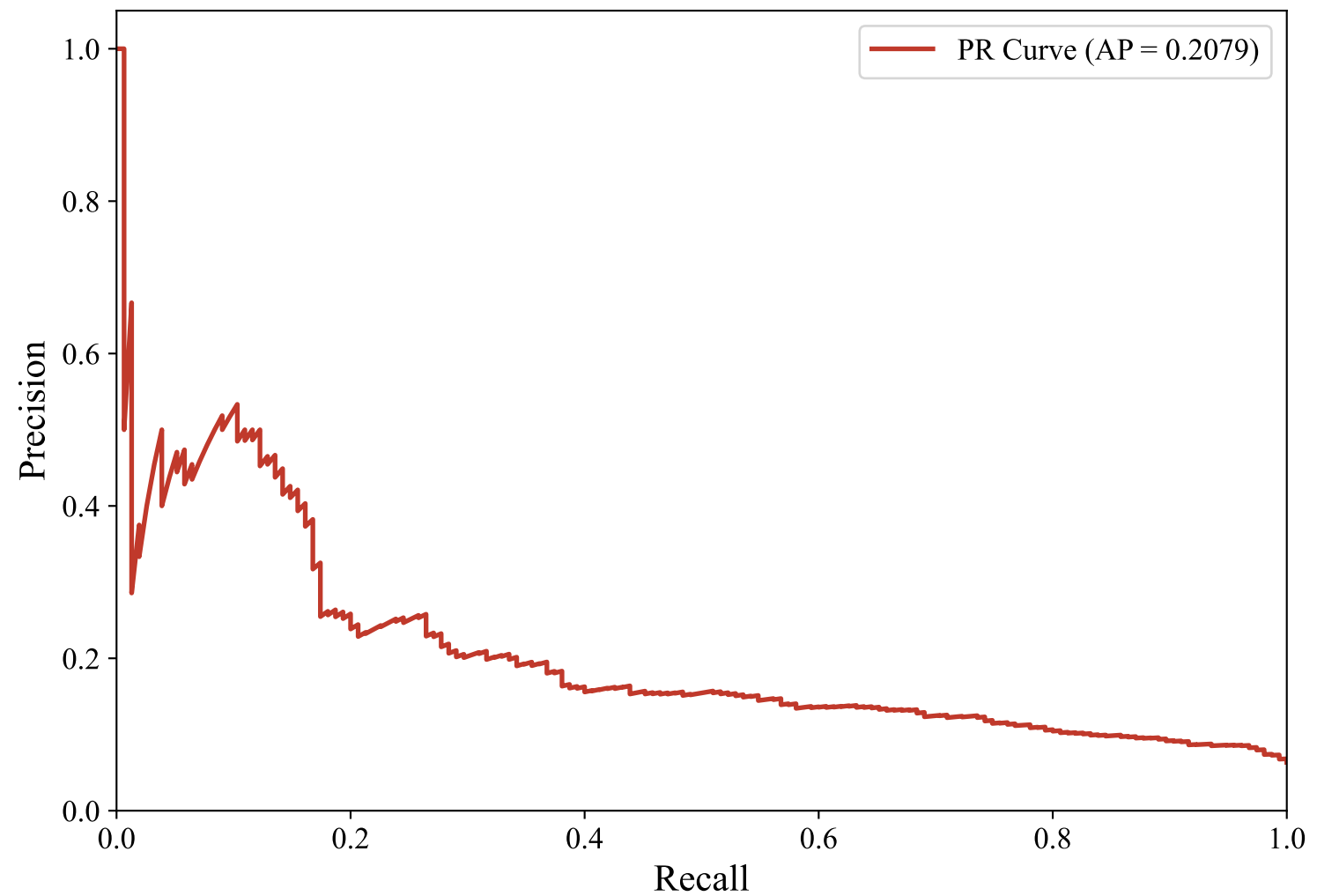
Precision-Recall Curve — SWEDISH_MANUAL (bert-base-multilingual-uncased, XGBoost)
