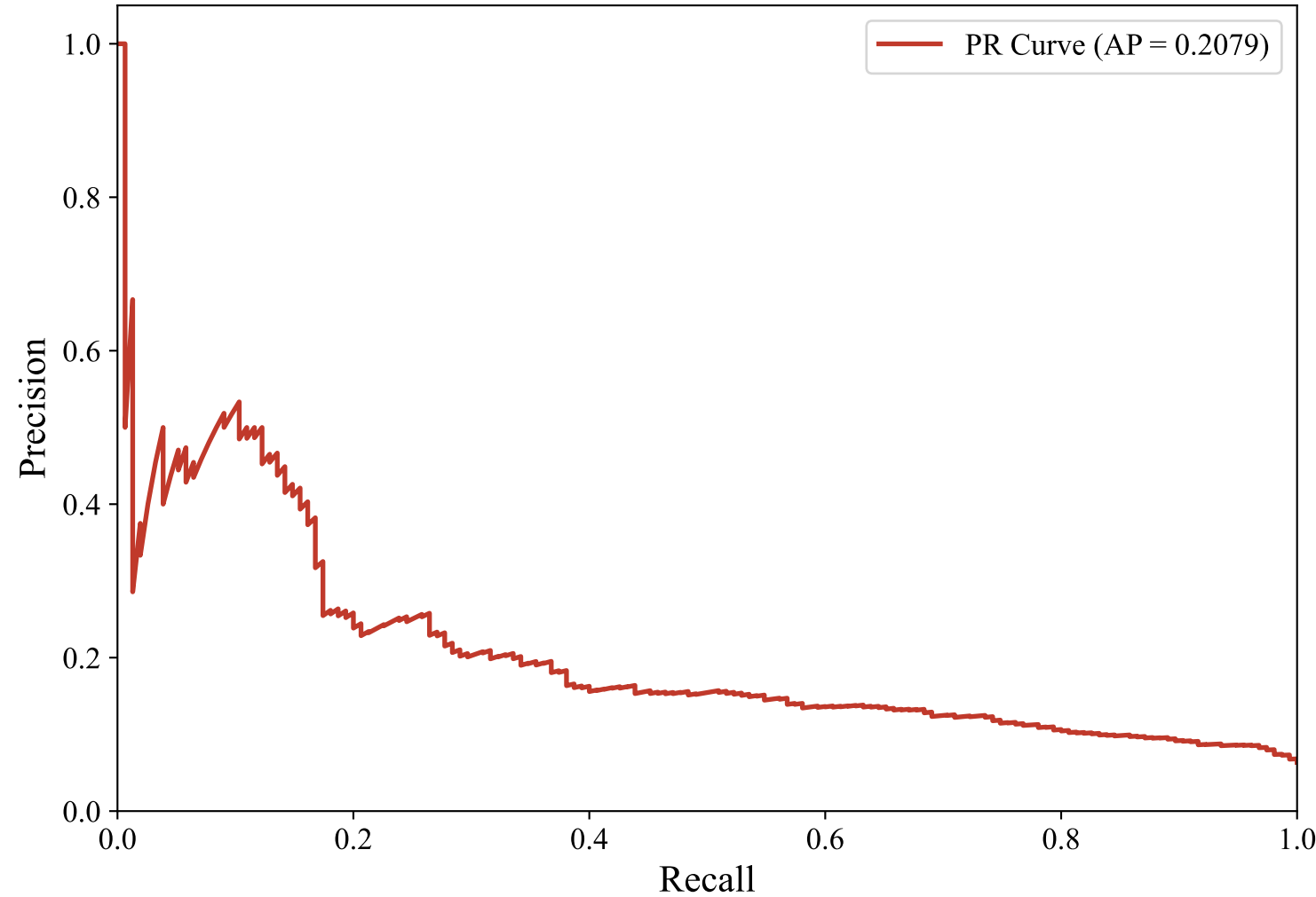
Precision-Recall Curve — SWEDISH_MANUAL (bert-base-multilingual-uncased, XGBoost_Optimized)
