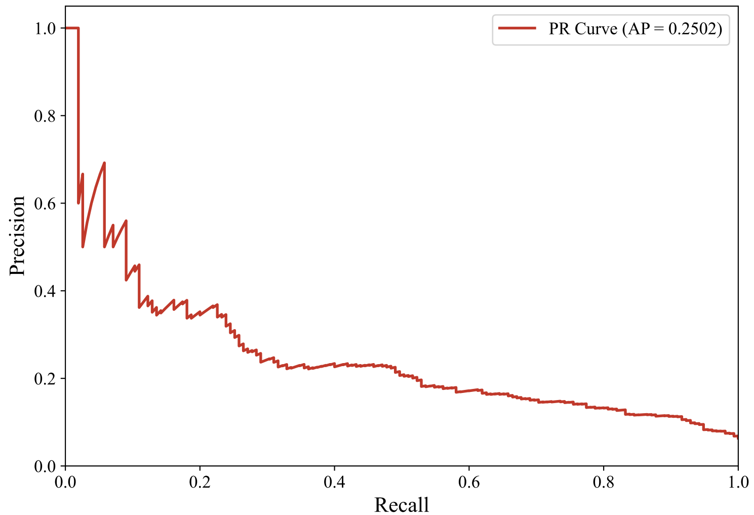
Precision-Recall Curve — SWEDISH_MANUAL (xlm-roberta-base, LightGBM_Optimized)
