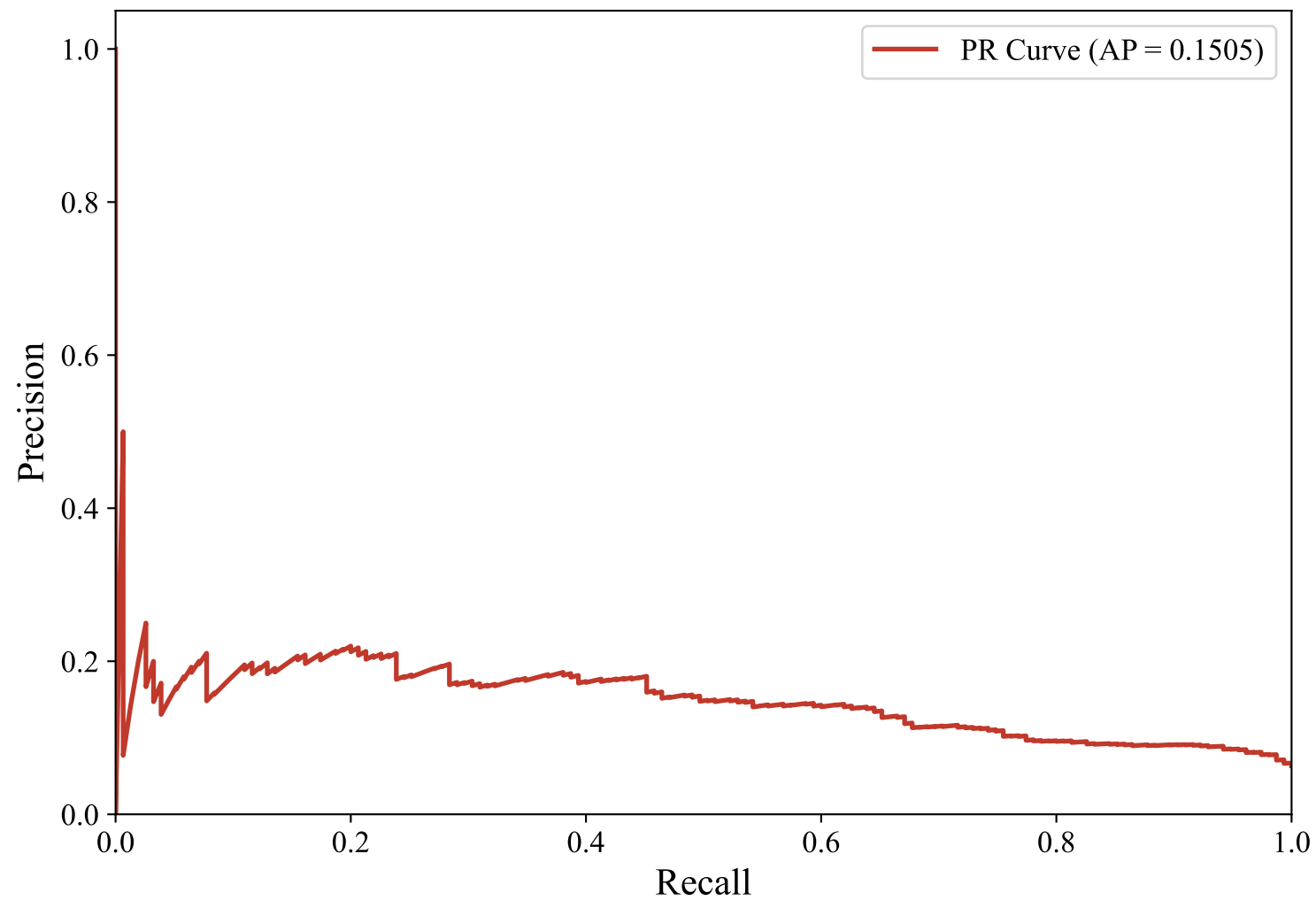
Precision-Recall Curve — SWEDISH_MANUAL (xlm-roberta-base, Random_Forest_Optimized)
