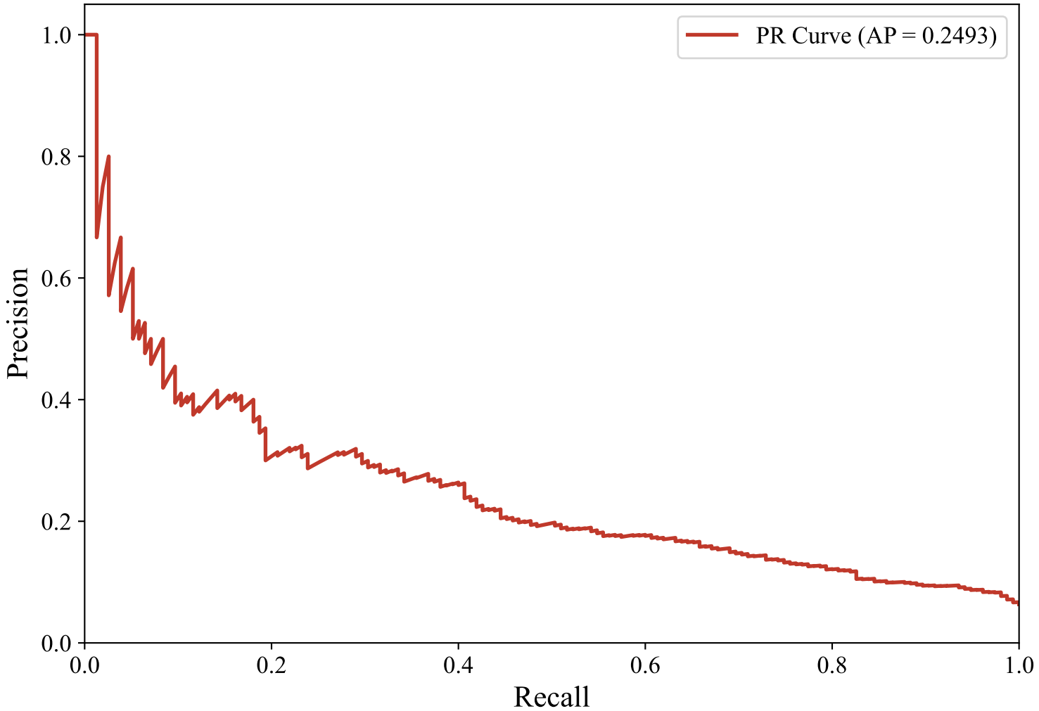
Precision-Recall Curve — SWEDISH_MANUAL (xlm-roberta-base, Voting_Ensemble)
