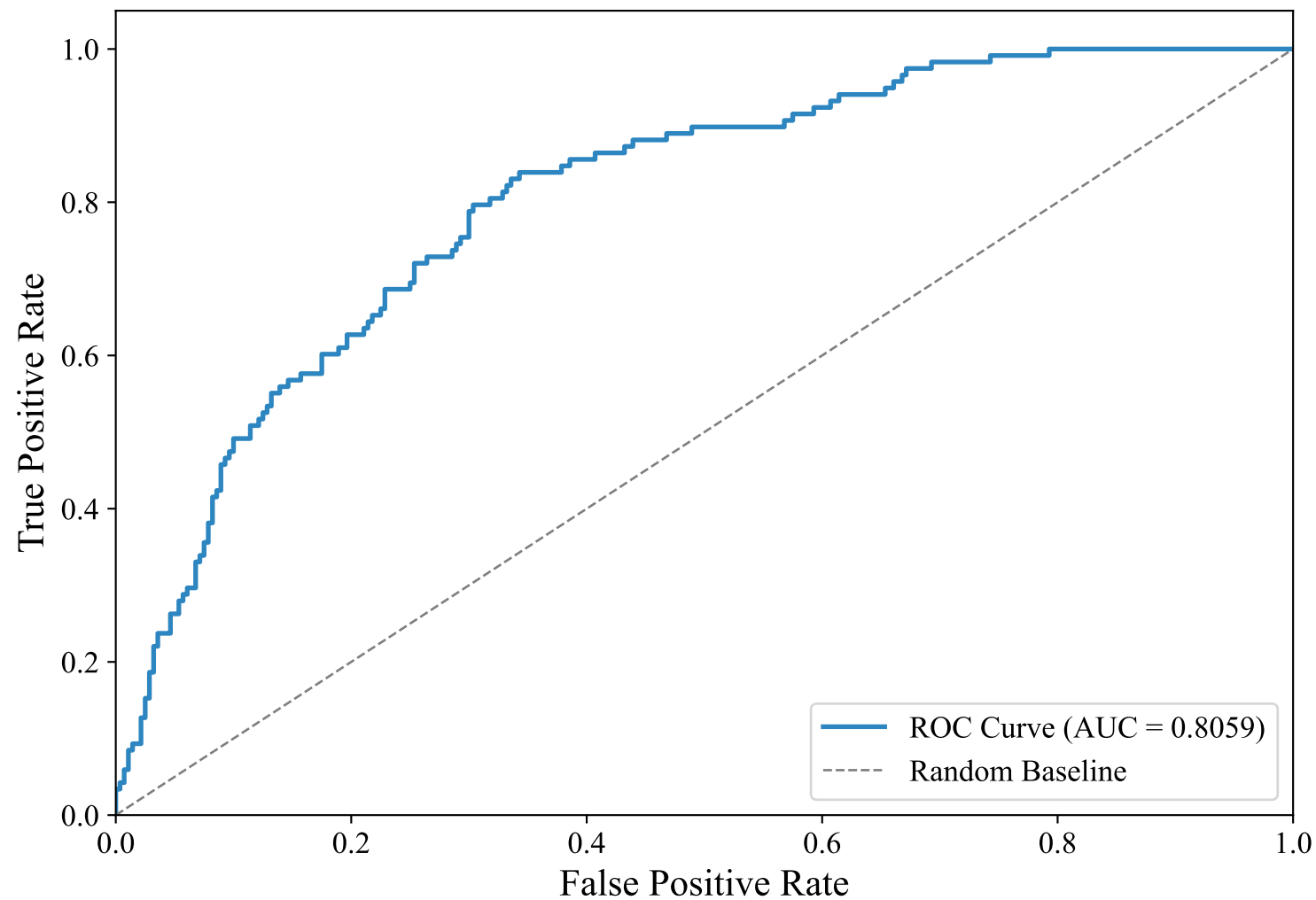
ROC Curve — DUTCH_MANUAL (xlm-roberta-base, LightGBM)
