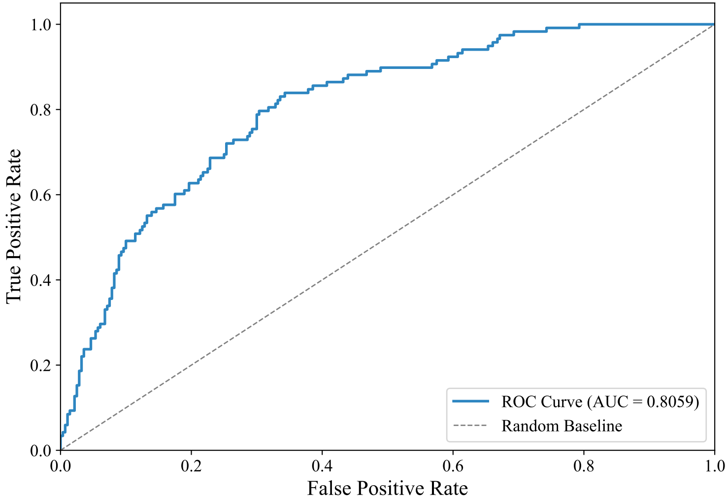
ROC Curve — DUTCH_MANUAL (xlm-roberta-base, LightGBM_Optimized)
