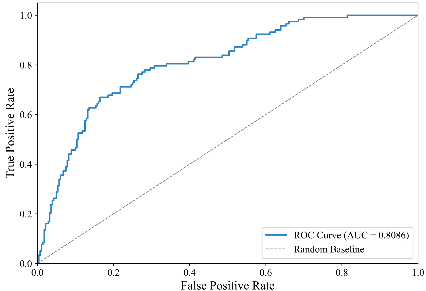
ROC Curve — DUTCH_MANUAL (xlm-roberta-base, XGBoost)
