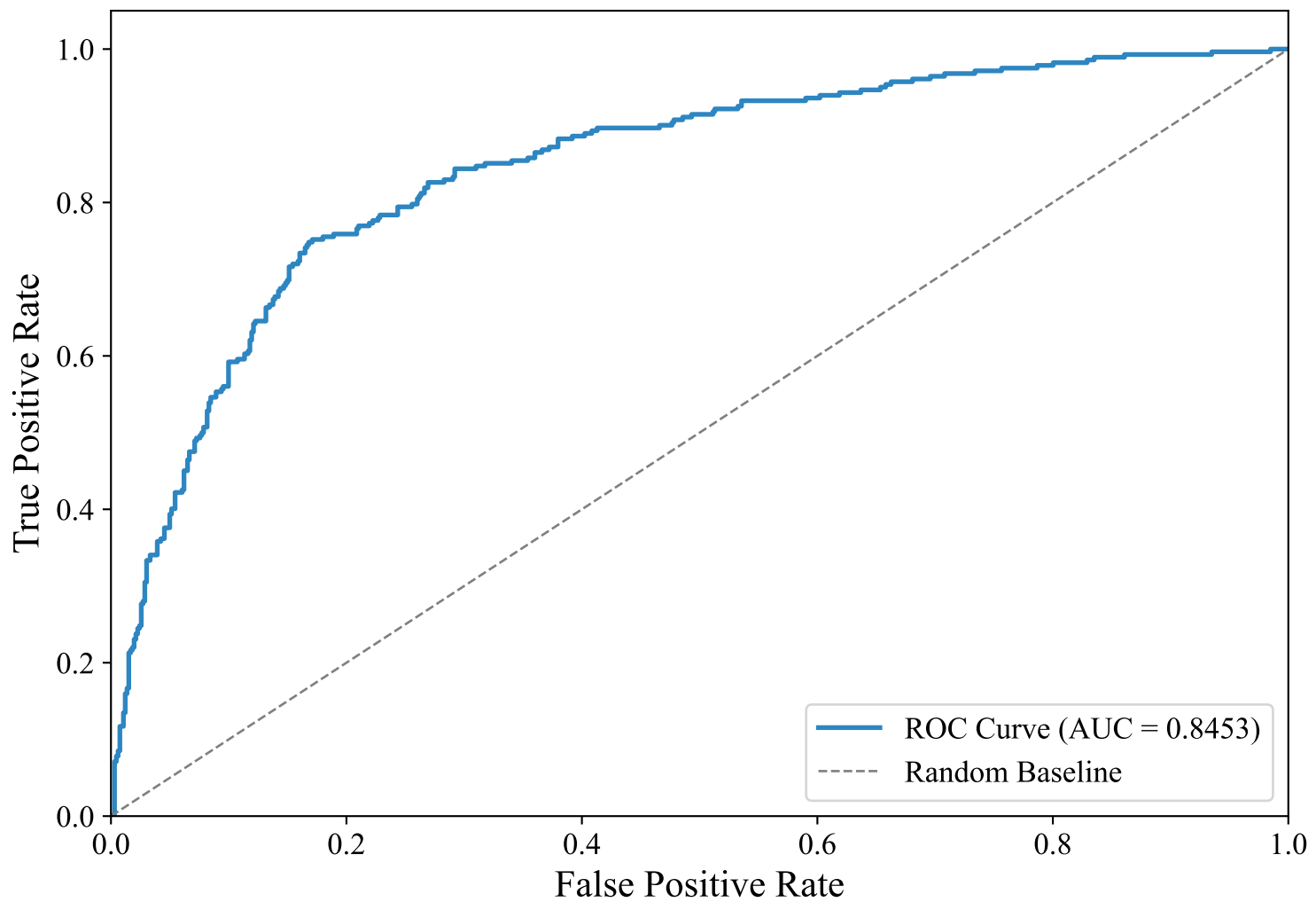
ROC Curve — ENGLISH_MANUAL (bert-base-multilingual-uncased, Voting_Ensemble)
