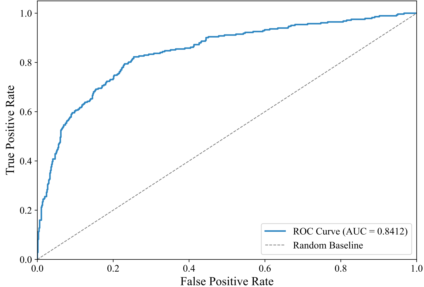
ROC Curve — ENGLISH_MANUAL (paraphrase-multilingual-mpnet-base-v2, Random_Forest_Optimized)
