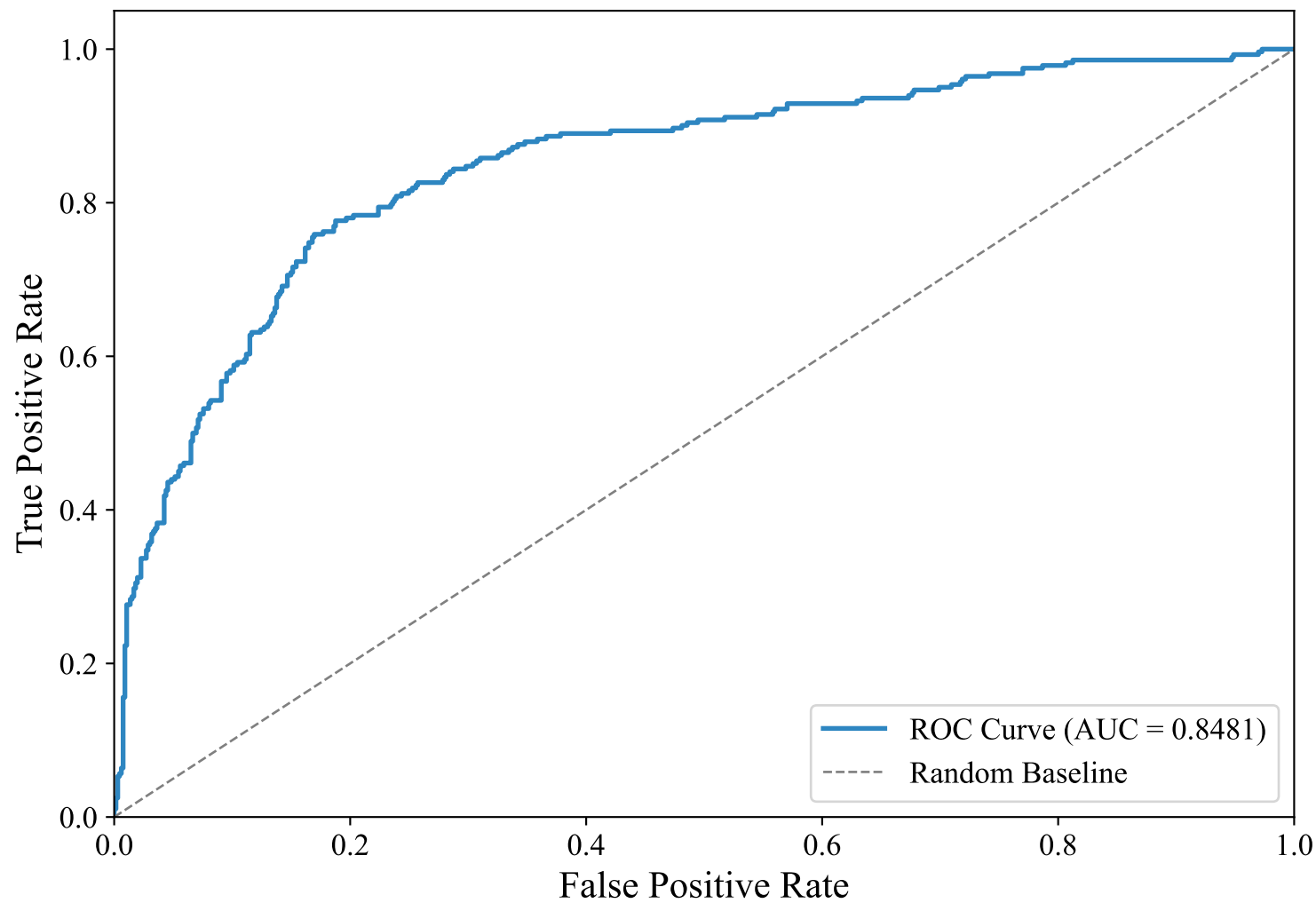
ROC Curve — ENGLISH_MANUAL (xlm-roberta-base, LightGBM_Optimized)
