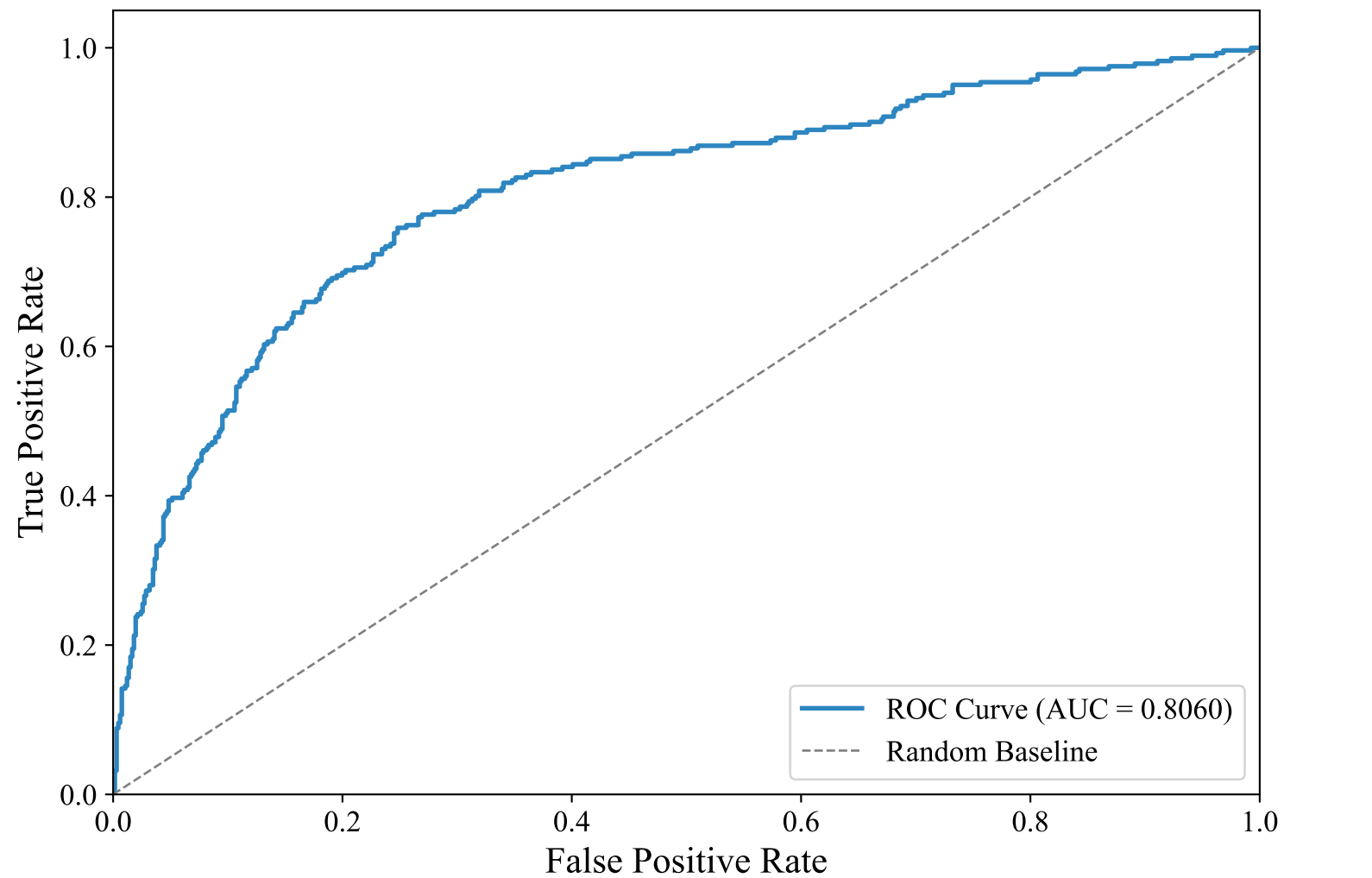
ROC Curve — ENGLISH_MANUAL (xlm-roberta-base, Random_Forest_Optimized)
