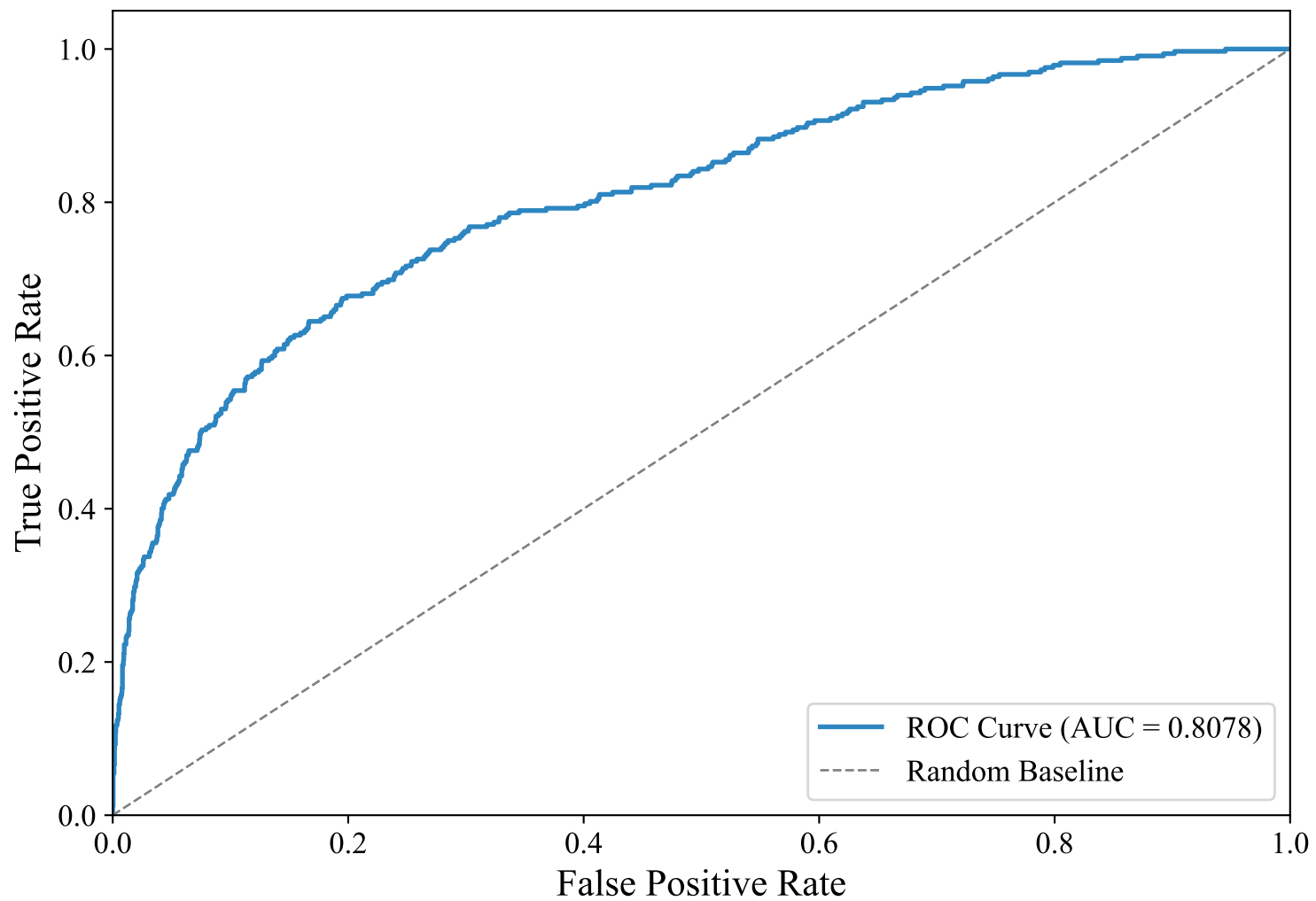
ROC Curve — GERMAN_MANUAL (paraphrase-multilingual-mpnet-base-v2, LightGBM)
