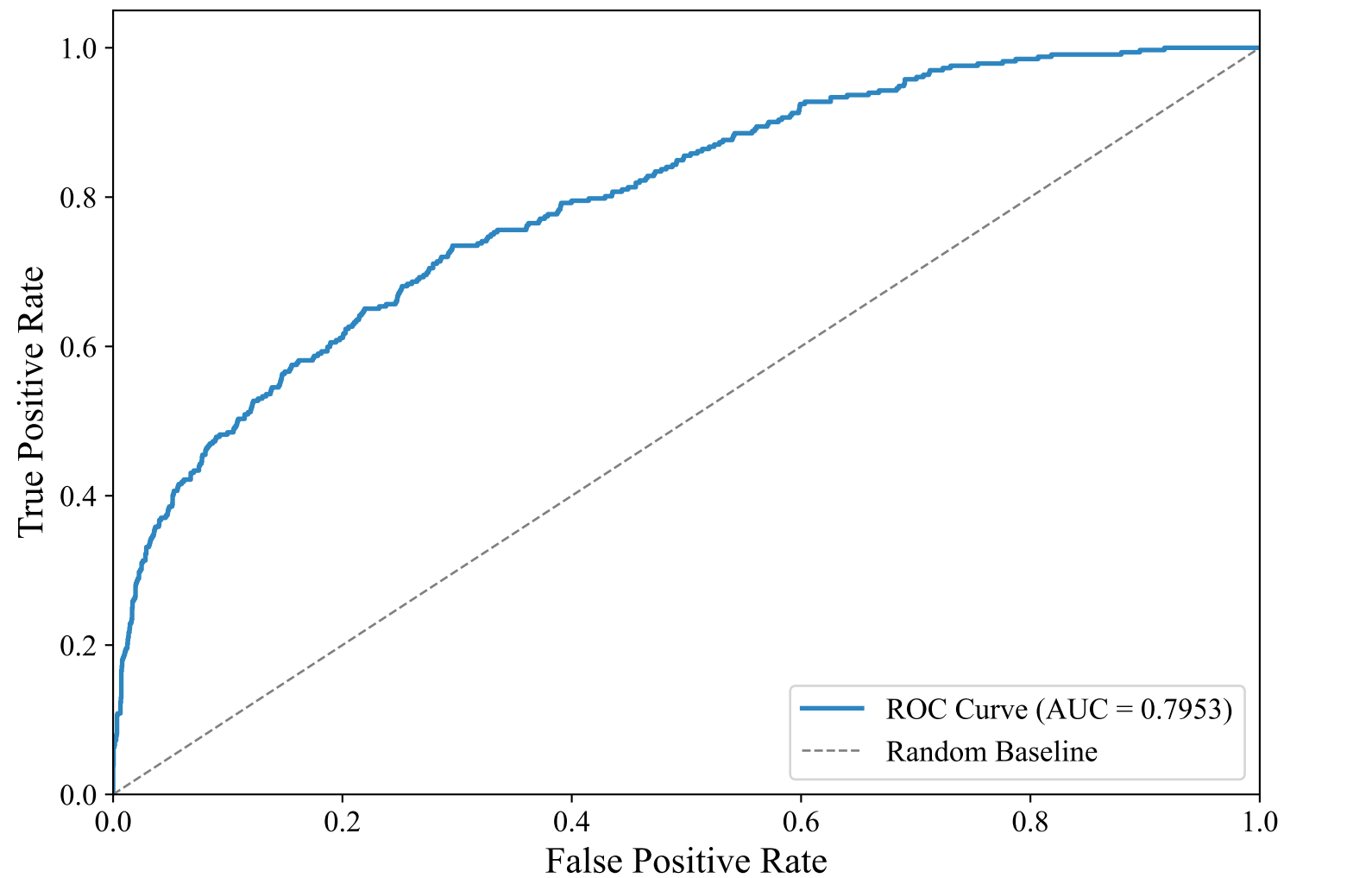
ROC Curve — GERMAN_MANUAL (xlm-roberta-base, Random_Forest_Optimized)
