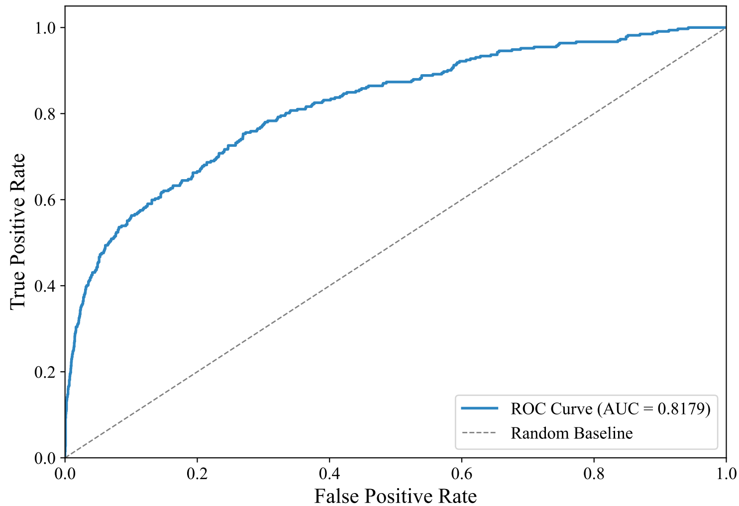
ROC Curve — GERMAN_MANUAL (xlm-roberta-base, XGBoost)
