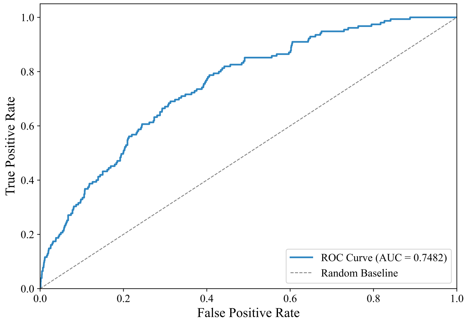
ROC Curve — SWEDISH_MANUAL (bert-base-multilingual-uncased, Voting_Ensemble)
