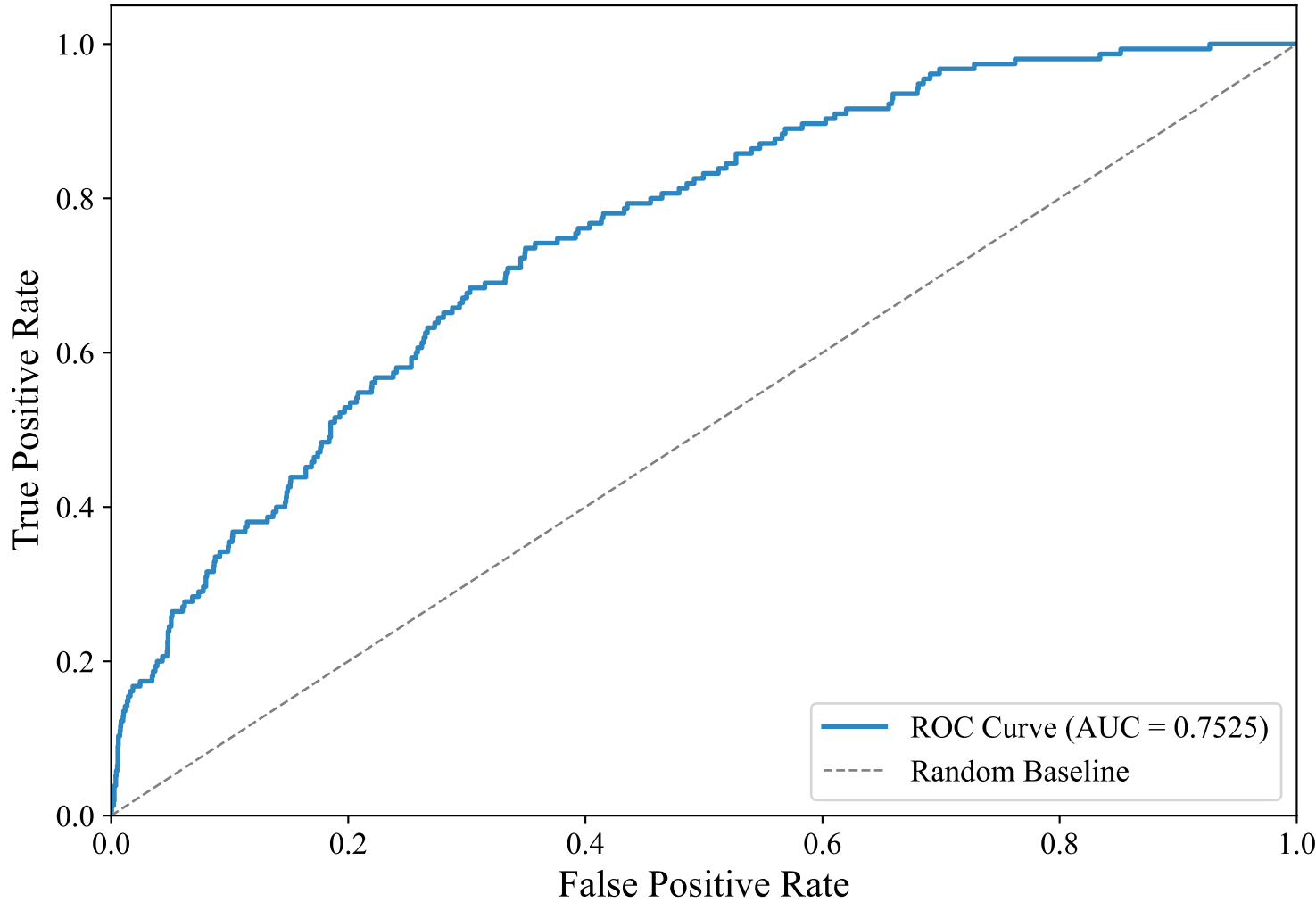
ROC Curve — SWEDISH_MANUAL (bert-base-multilingual-uncased, XGBoost)
