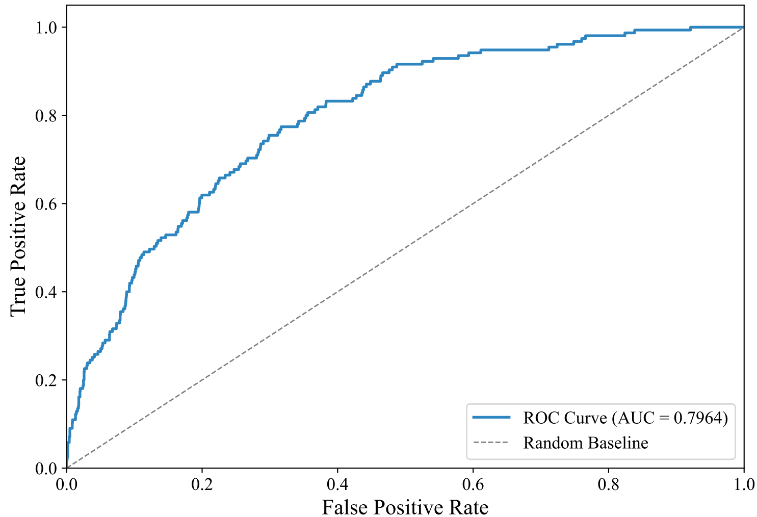
ROC Curve — SWEDISH_MANUAL (xlm-roberta-base, LightGBM)
