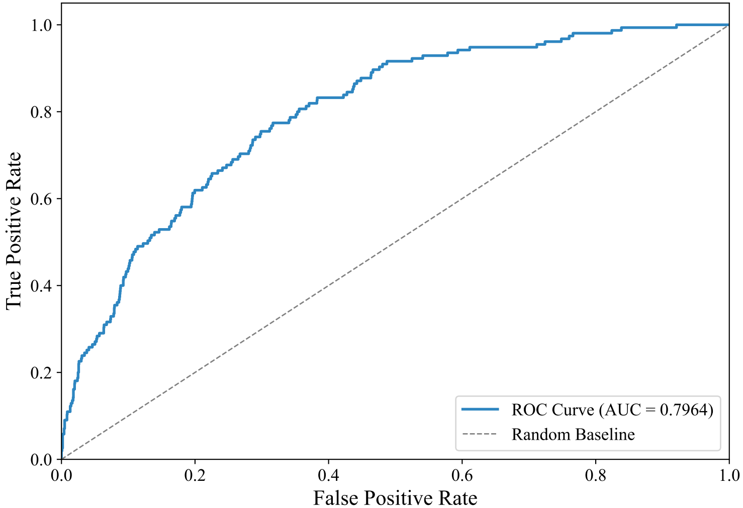
ROC Curve — SWEDISH_MANUAL (xlm-roberta-base, LightGBM_Optimized)
