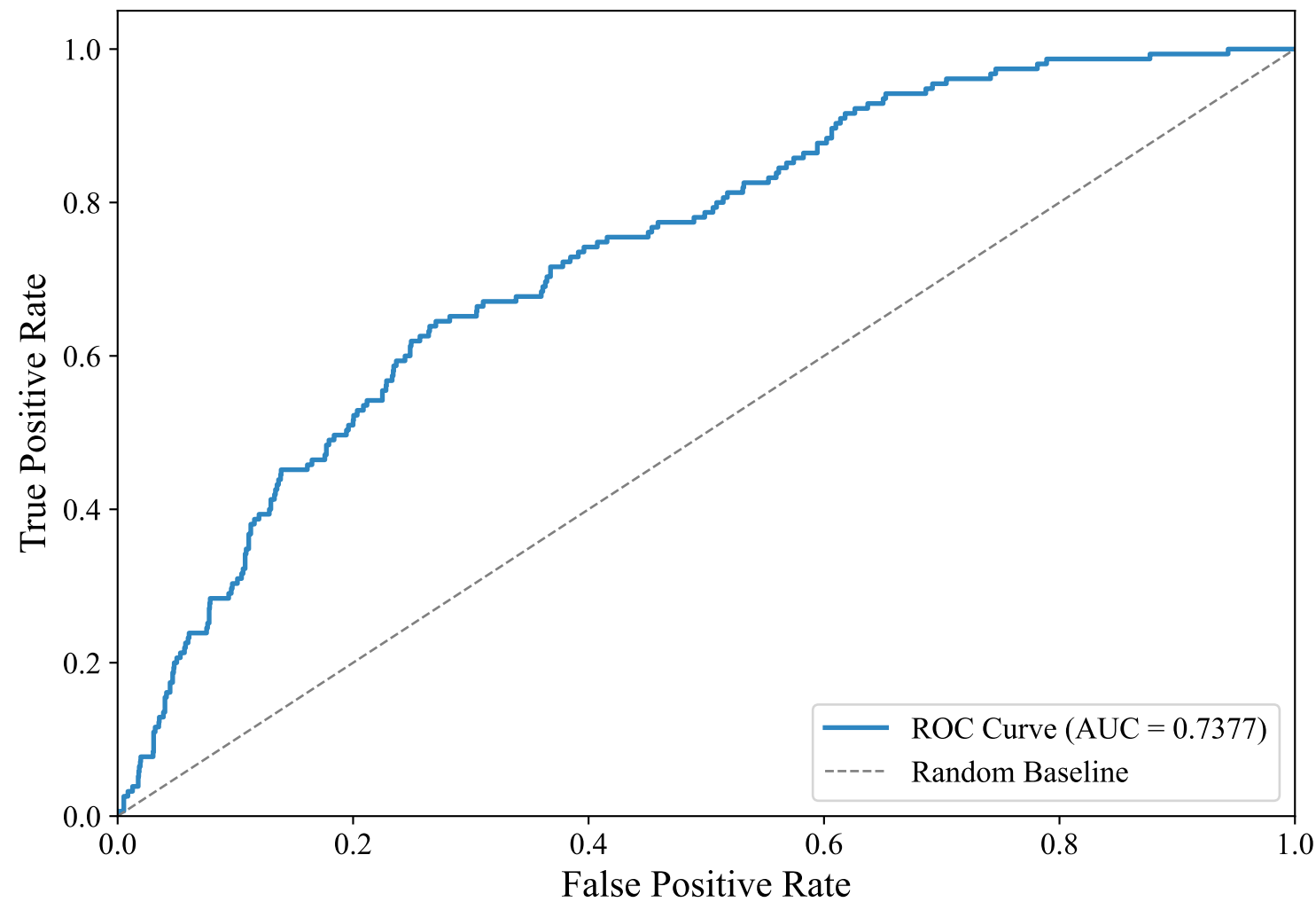
ROC Curve — SWEDISH_MANUAL (xlm-roberta-base, Random_Forest_Optimized)
