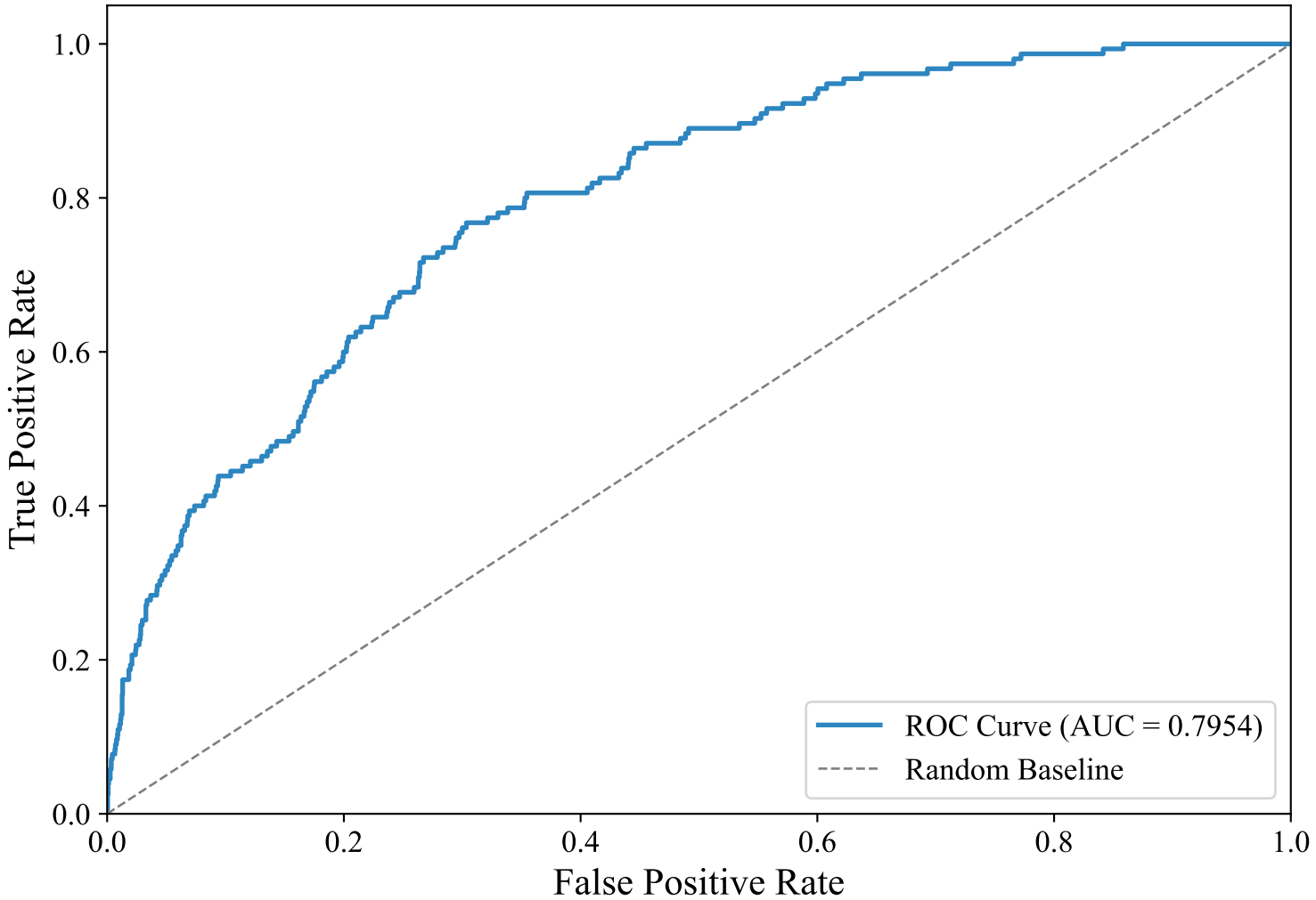
ROC Curve — SWEDISH_MANUAL (xlm-roberta-base, XGBoost_Optimized)
