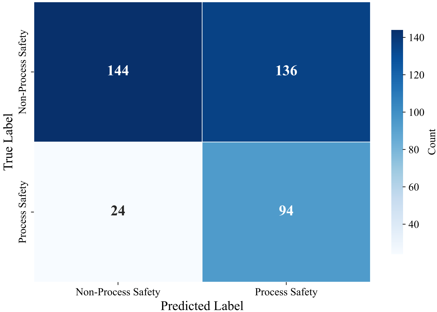
Confusion Matrix — DUTCH_MANUAL (bert-base-multilingual-uncased, Random_Forest)
