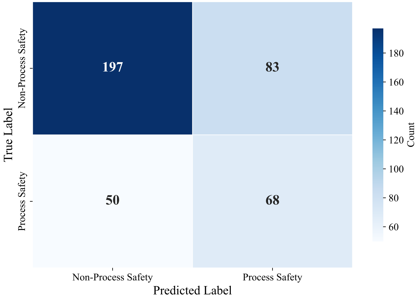
Confusion Matrix — DUTCH_MANUAL (bert-base-multilingual-uncased, SVM)
