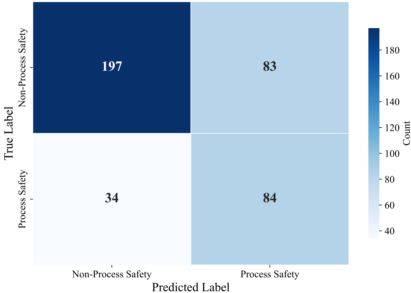
Confusion Matrix — DUTCH_MANUAL (bert-base-multilingual-uncased, XGBoost_Optimized)
