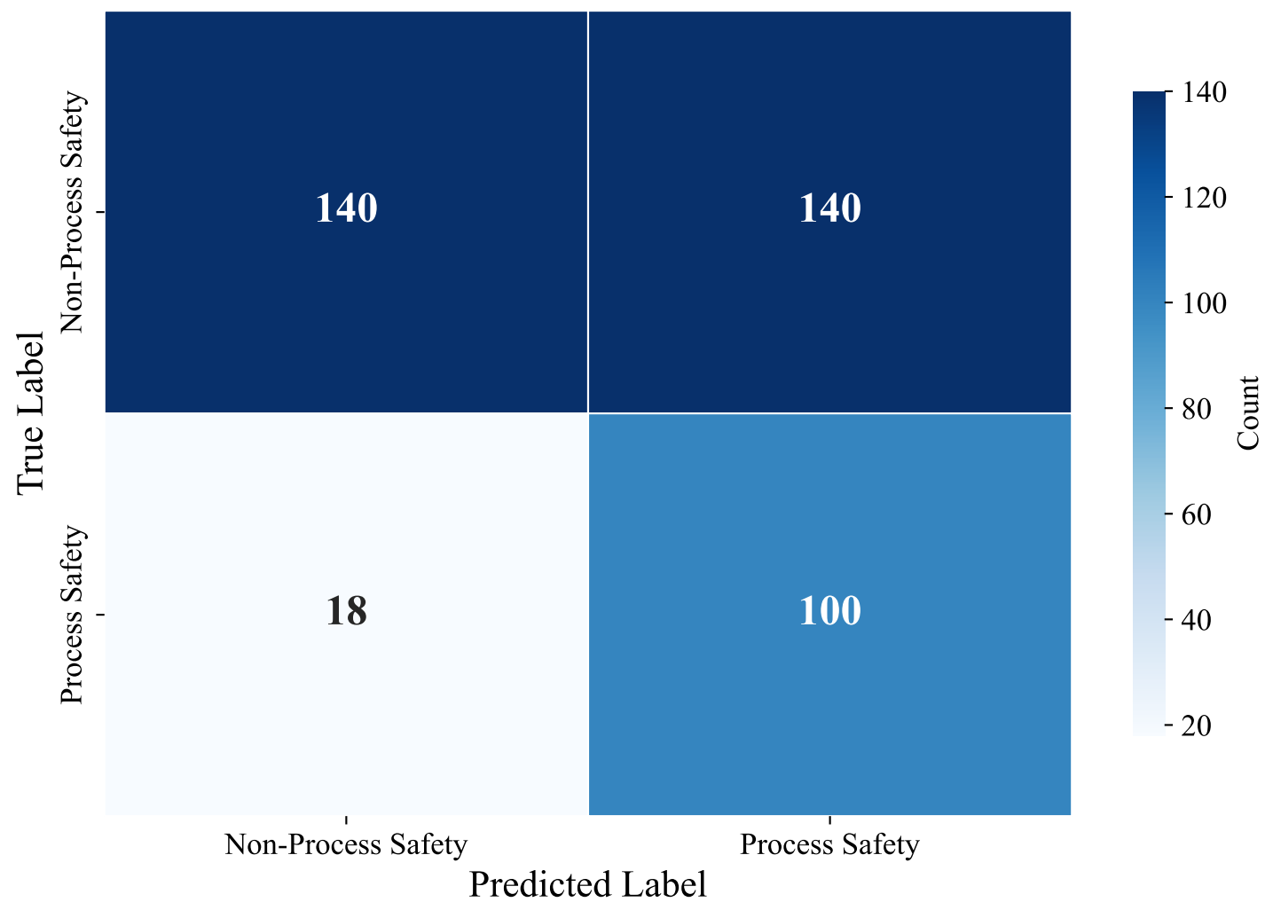
Confusion Matrix — DUTCH_MANUAL (efederici/e5-base-multilingual-4096, Random_Forest)
