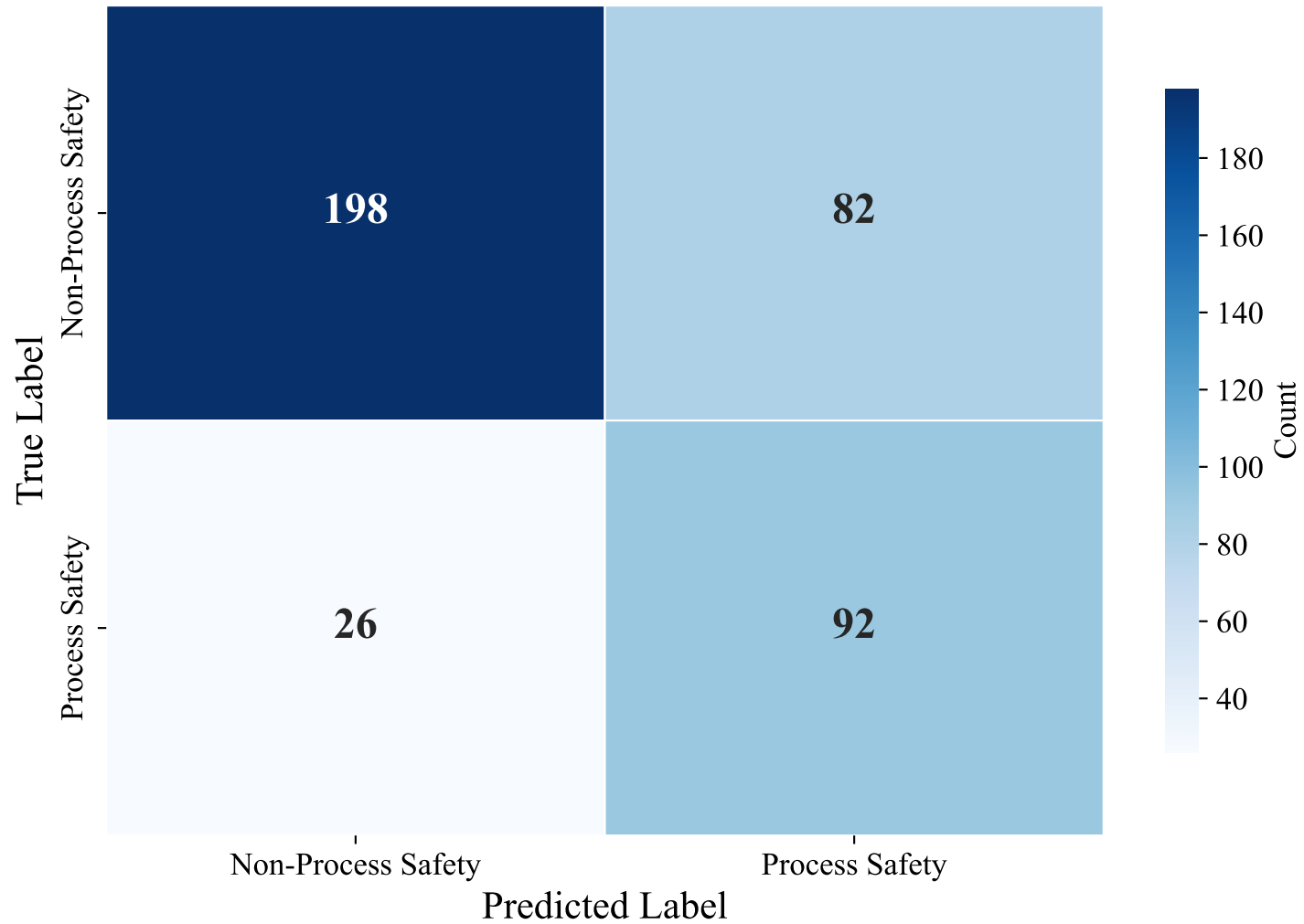
Confusion Matrix — DUTCH_MANUAL (efederici/e5-base-multilingual-4096, XGBoost)
