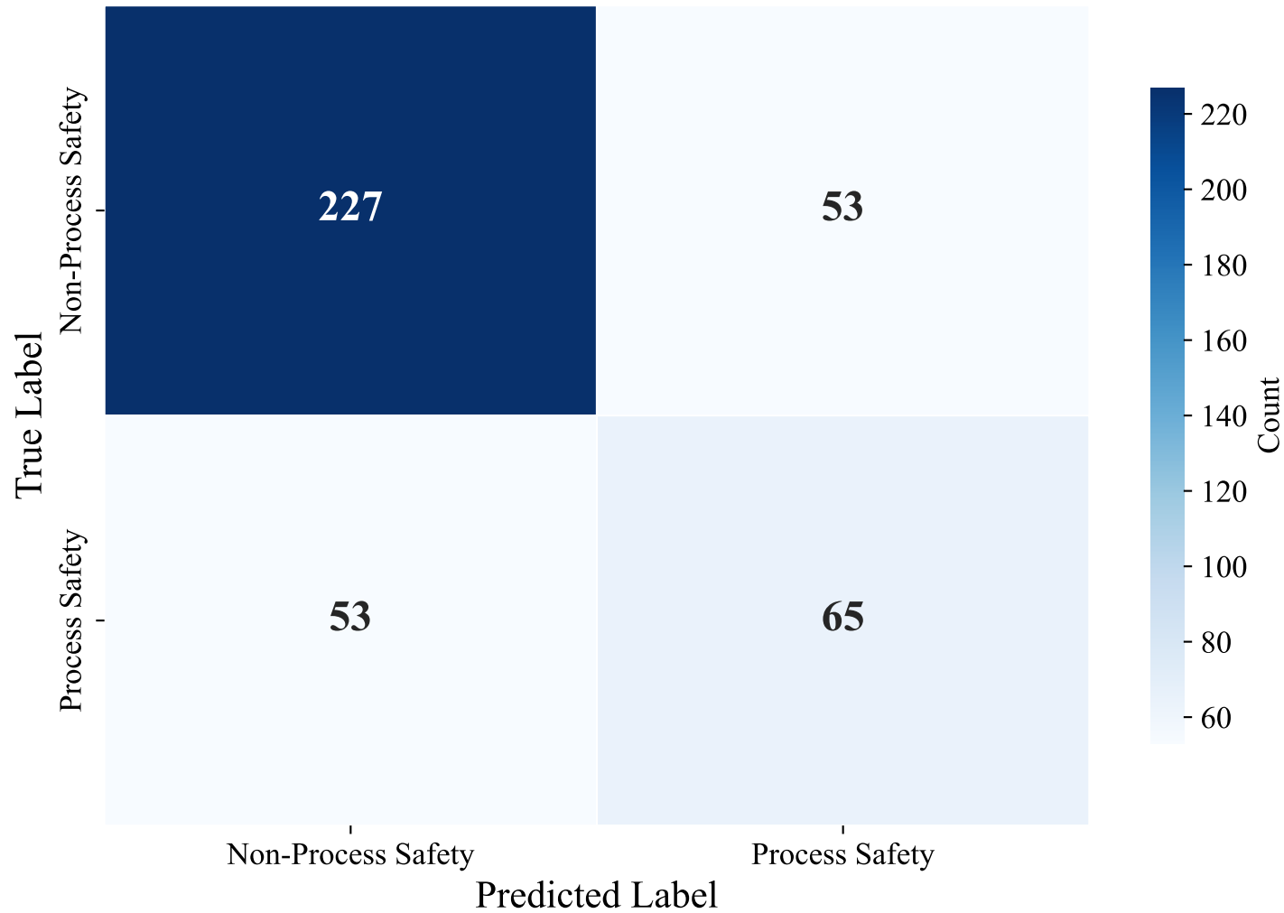
Confusion Matrix — DUTCH_MANUAL (intfloat/multilingual-e5-large-instruct, SVM)
