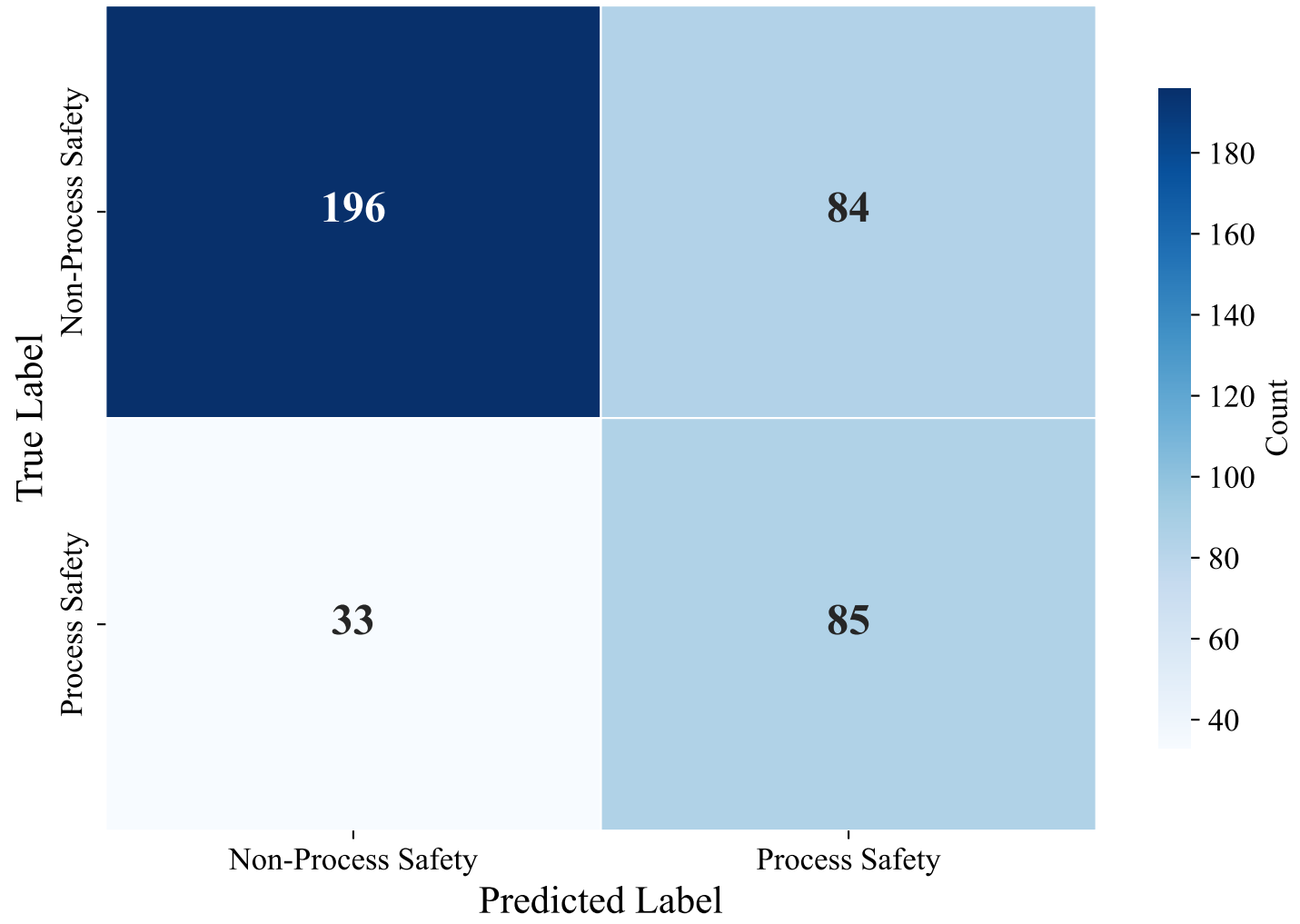
Confusion Matrix — DUTCH_MANUAL (paraphrase-multilingual-MiniLM-L12-v2, Voting_Ensemble)
