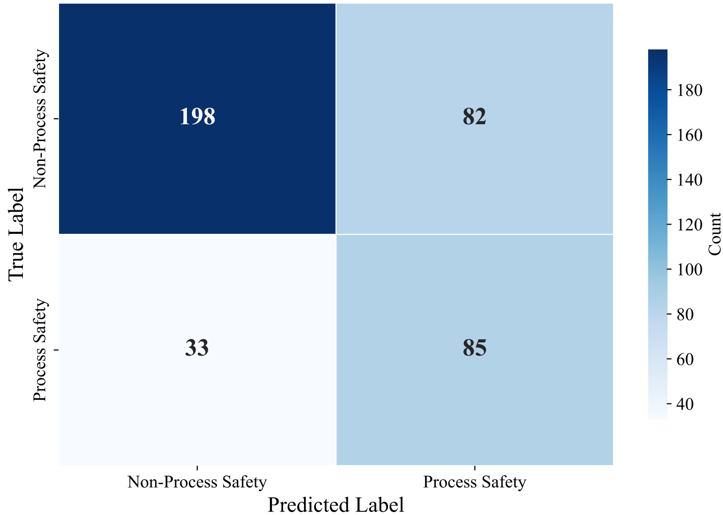
Confusion Matrix — DUTCH_MANUAL (paraphrase-multilingual-MiniLM-L12-v2, XGBoost_Optimized)
