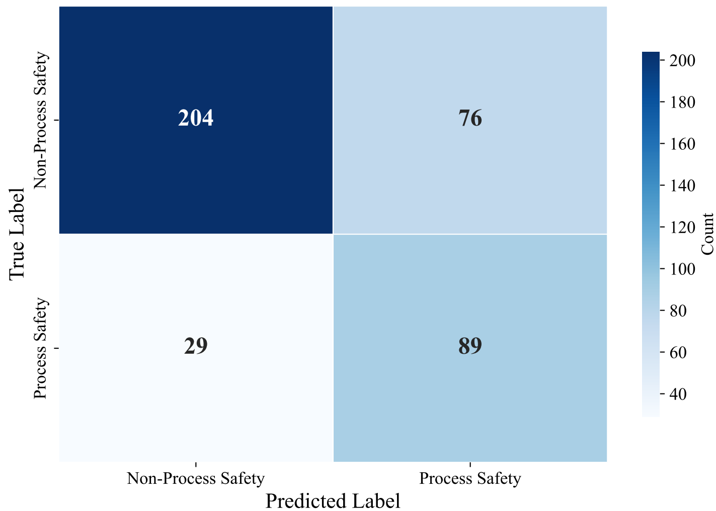
Confusion Matrix — DUTCH_MANUAL (paraphrase-multilingual-mpnet-base-v2, LightGBM)
