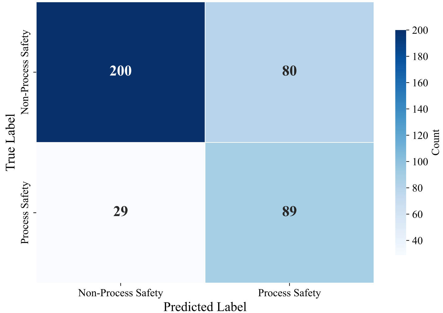
Confusion Matrix — DUTCH_MANUAL (paraphrase-multilingual-mpnet-base-v2, Voting_Ensemble)
