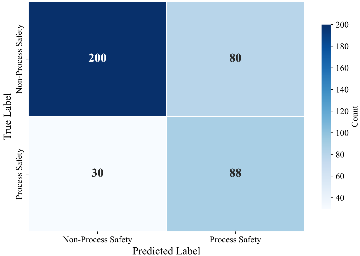
Confusion Matrix — DUTCH_MANUAL (paraphrase-multilingual-mpnet-base-v2, XGBoost)
