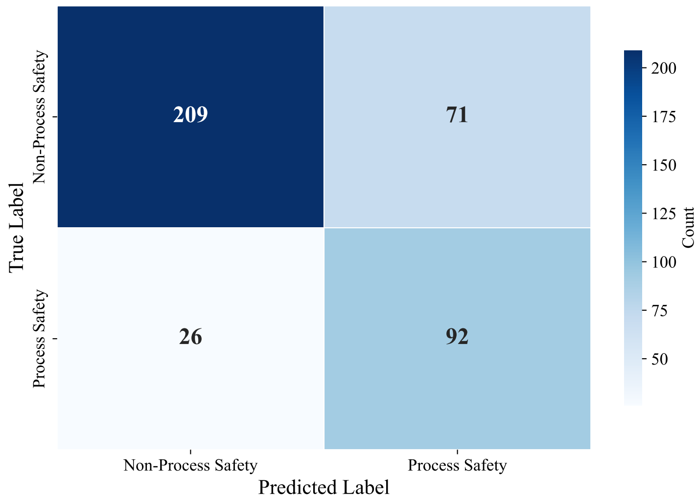
Confusion Matrix — DUTCH_MANUAL (upskyy/bge-m3-korean, LightGBM)
